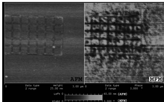
Figure 3, above: AFM/MFM image of 300 nm pattern. Images show the same area.
