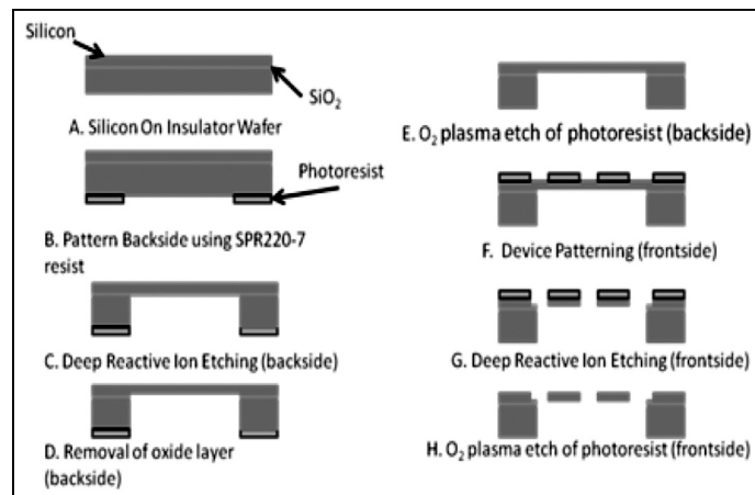
Figure 2: Schematic of the fabrication steps used to fabricate the free standing devices.
