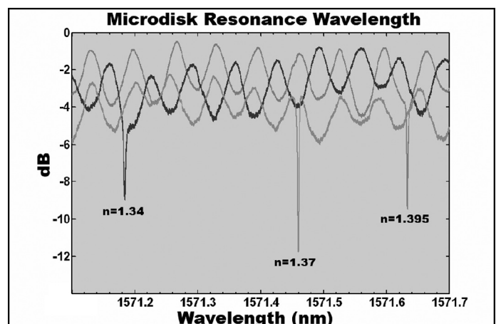
Figure 2: Microdisk spectral response.
