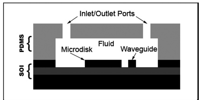
Figure 1: Resonator integrated with microfluidic channel. (Resonator radius: 20 \mu\text{m} , height: 230 nm.)
