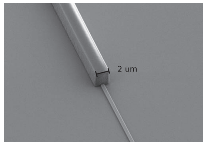
Figure 2: Fabricated waveguides.
