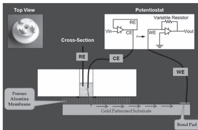
Figure 2, below: Electrodeposition experimental setup includes: potentiostat circuit, three electrodes, membrane on patterned gold substrate, and potassium aurocyanide.
