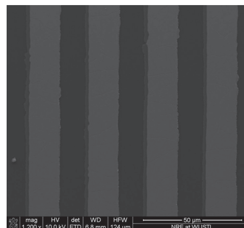
Figure 2: SEM image of 20\ \mu\text{m} wire and 10\ \mu\text{m} space pixel.
