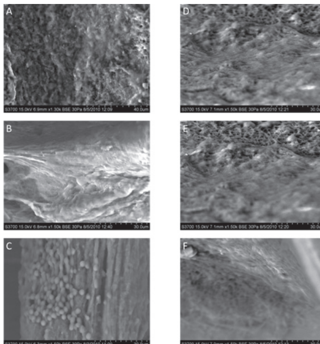
Figure 3: Representative SEMs of thrombus at different shear rates, 10,000\text{ s}^{-1} (A), 4,000\text{ s}^{-1} (B), 500\text{ s}^{-1} (C), and different regions of a 10,000\text{ s}^{-1} clot, downstream (D, E), and upstream corner (F). Flow is toward the top of the page in all cases.
