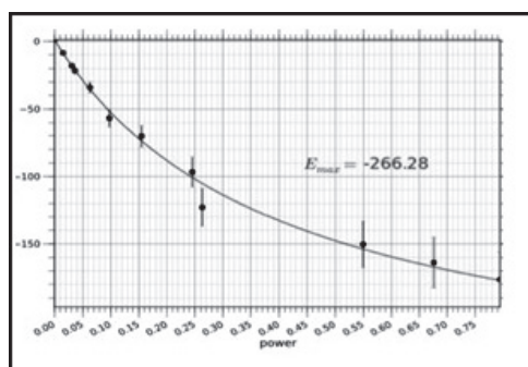
Figure 3: Measurement of DNP enhancement of signal from 140 mM CAT 1 .
