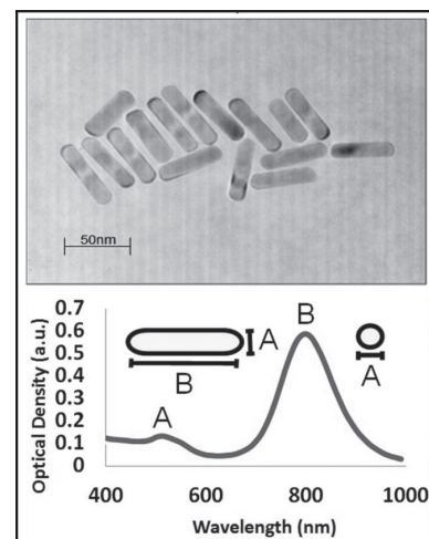
Figure 2: (a) TEM of as-synthesized GNRs, and (b) Typical absorbance spectra of as synthesized GNRs.
