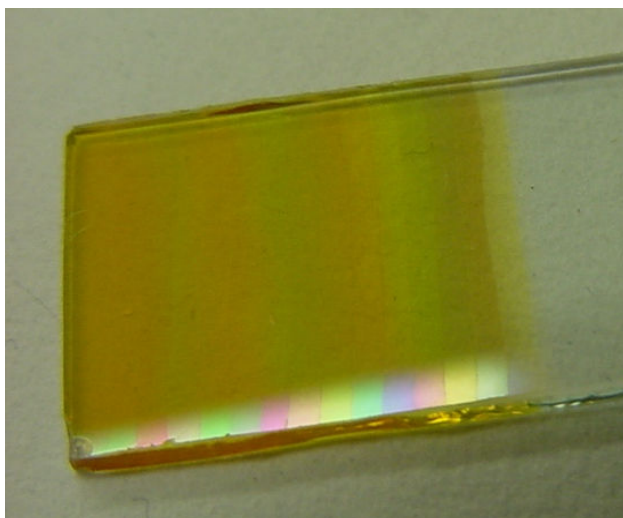
Figure 4. Cuprous oxide ( \text{Cu}_2\text{O} ) electrodeposited from the electrolyte in a rainbow pattern, the end goal of the challenge. It would be nice if the students could make the patterns in the correct order, or perhaps, by proper masking, draw shapes and designs in color.
