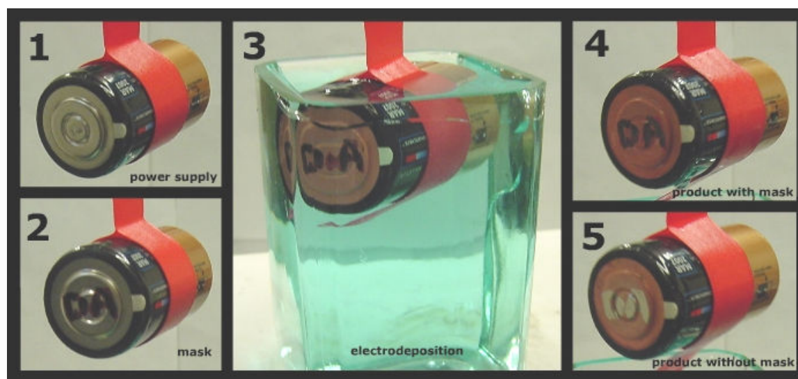
Figure 2. The most simple demonstration of an electrodeposition process (the electrolysis of copper sulfate to copper metal). The initials DA are drawn using a permanent marker (not water-soluble, not conducting) as a mask so that the initial battery terminal surface is revealed. Note that the copper deposition proceeds on the negative side (where electrons meet copper cations, based on \text{Cu}^{2+}_{\text{aqueous}} + 2\text{e}^{-}_{\text{electrode}} \rightarrow \text{Cu}_{\text{metal}} . (0.2 M sulfuric acid, 0.2 M cupric sulfate pentahydrate, 1-2 minutes: CAUTION, mildly corrosive bath)
