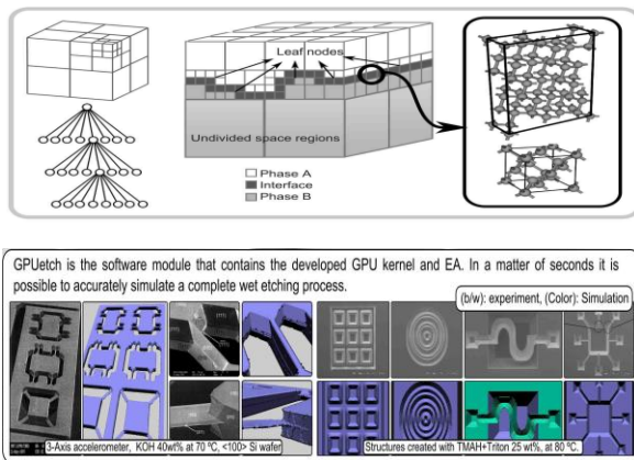
Figure 1: Schematic illustration of physical mechanisms addressed by the code. 1-3
