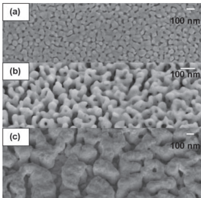
Figure 1: SEM images of nanoporous gold; (a) etched in 15% v/v \text{HNO}_3 , (b) etched in 20% v/v \text{HNO}_3 (imaged at an angle), and (c) after 9 hours of annealing at 450°C (imaged at an angle).
