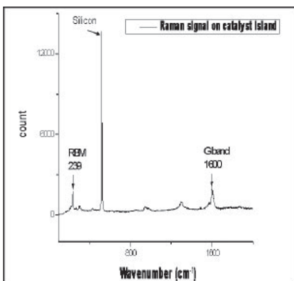
Figure 3: Raman spectrum data of the catalyst island.
