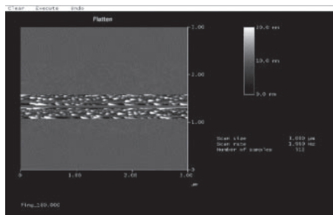
Figure 4: AFM image of a good lift off between the two stems.
