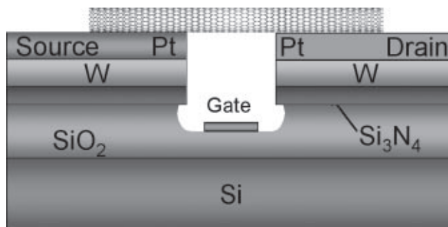
Figure 1: Suspended device structure.
