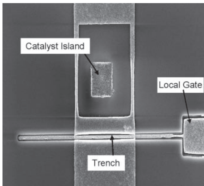
Figure 2: Suspended device with the catalyst island patterned on top of the nitride.
