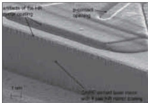
Etched facet laser
