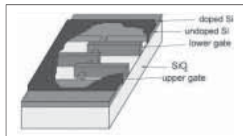
Figure 1: Schematic of single-electron tunneling multi-gate device
