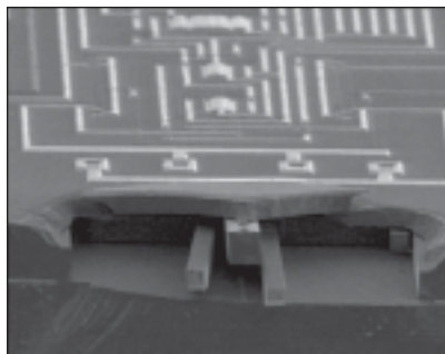
Single crystal Si encapsulation layer allows CMOS integration.
