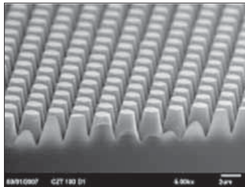
Motheye Graded Index Antireflection Structure etched into CdZnTe substrate for radiation hard LWIR applications
